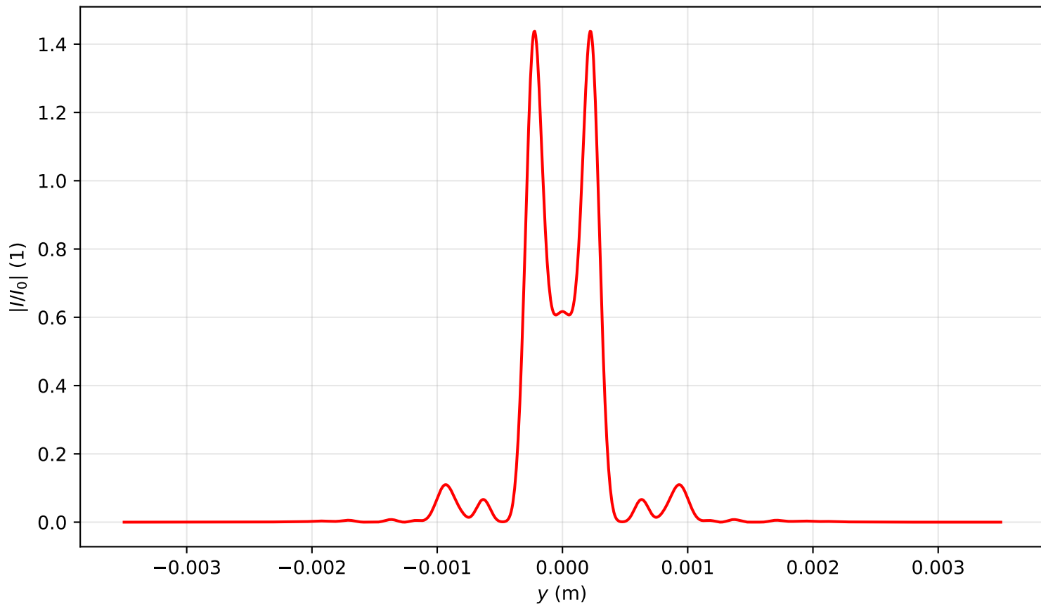
Intensity profile I(x=0, y, z=1.194)/I_0 , \text{Pin}=6.0\text{Pcr} , artificial time
